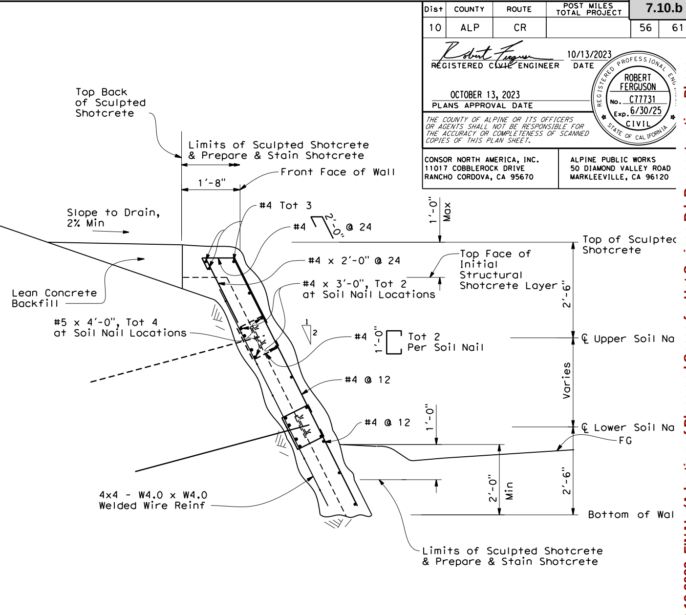
SINGLE ANCHOR TYPICAL SECTION 3/4"=1'-0"
