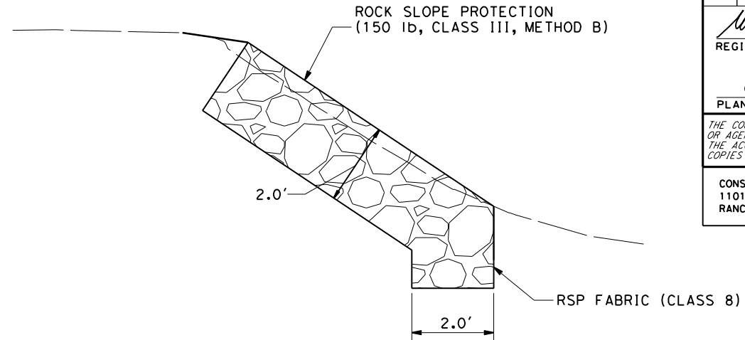
RSP DETAIL NO SCALE
