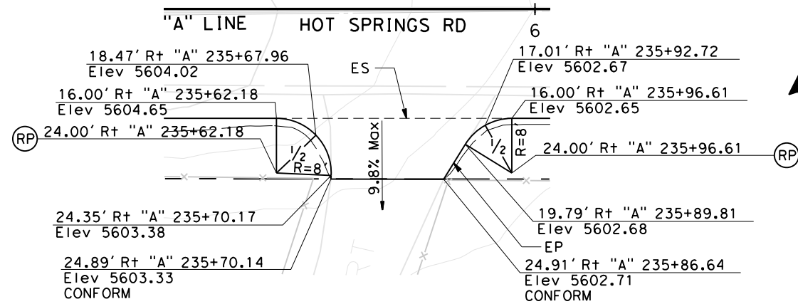
DRIVEWAY 10 Sta "A" 235+62.18 TO 235+96.61 R+ SCALE: 1"=10'
