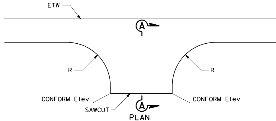
TYPICAL DRIVEWAY DETAIL NO SCALE
