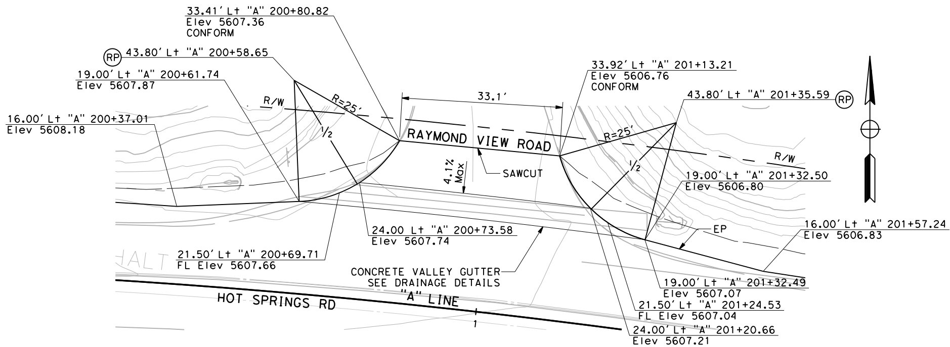
HOT SPRINGS Rd AT RAYMOND VIEW Rd SCALE: 1"=10'
