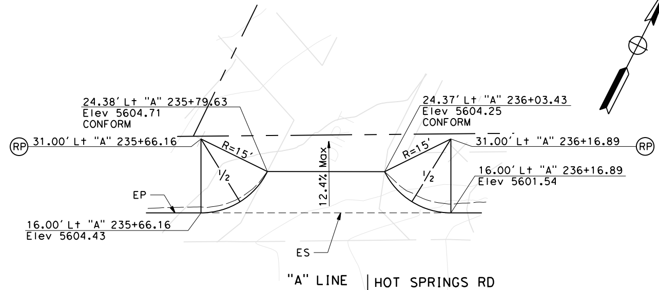
DRIVEWAY 11 Sta "A" 235+66.18 TO 236+16.89 Rt SCALE: 1"=10'
