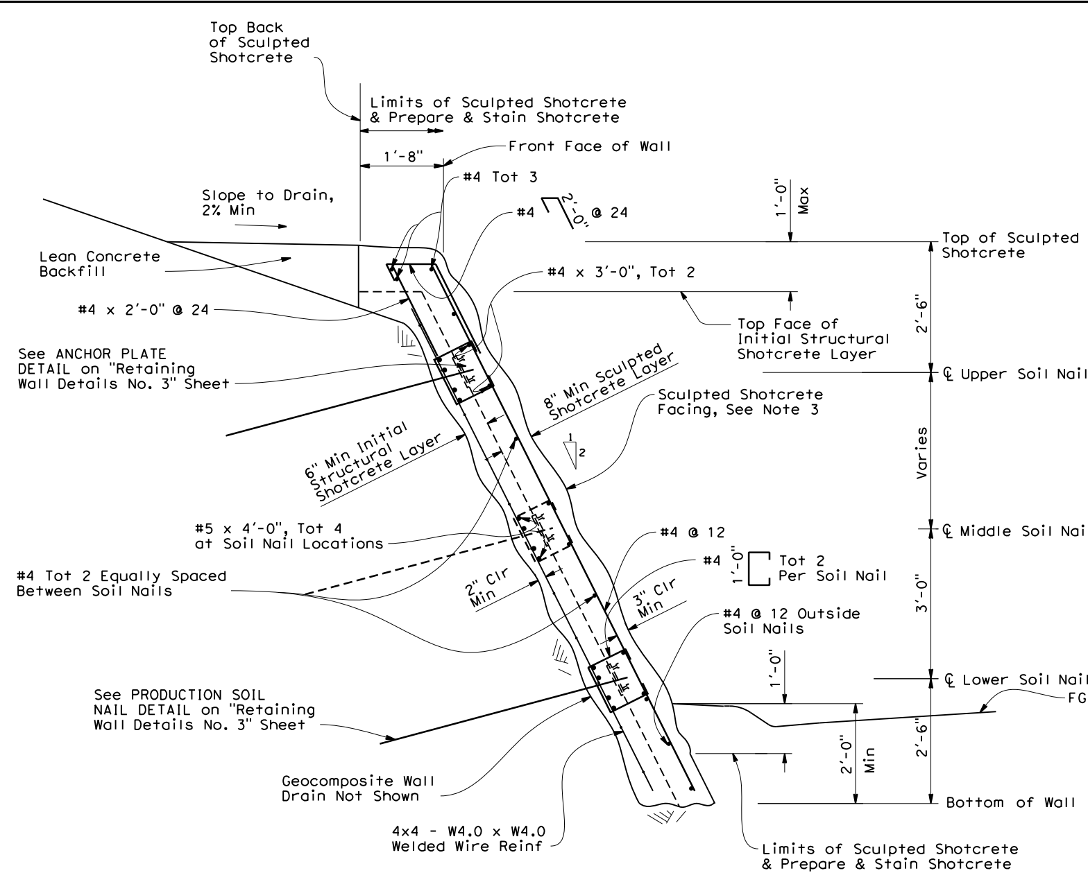
DOUBLE ANCHOR TYPICAL SECTION 3/4"=1'-0"
