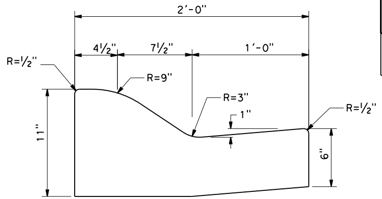
Conc CURB AND GUTTER NO SCALE
