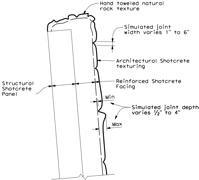
TYPICAL SECTION 1"=1'-0"
